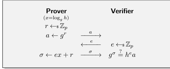
Figure 1: Schnorr \Sigma -Protocol for DLog Language.
